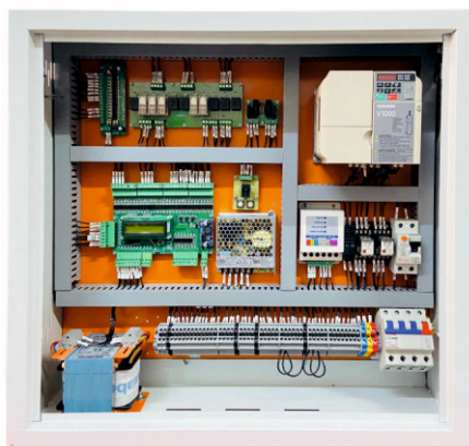
Elevator Geared Controller
